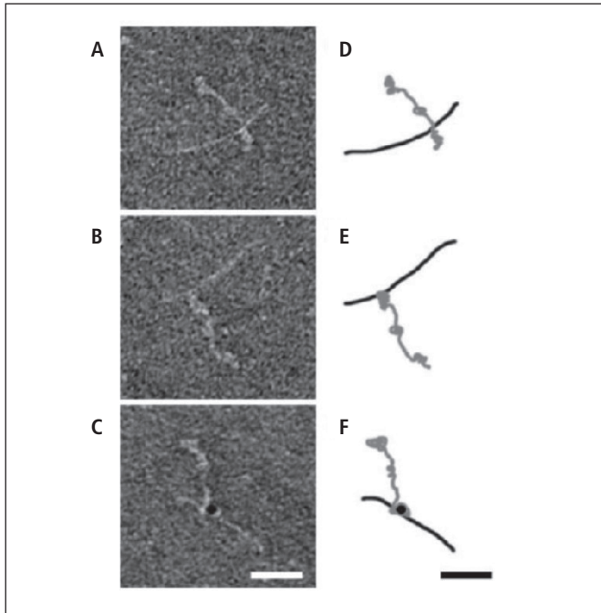
Figure 3: Electron micrographic visualisation of FXIII-mediated cross-linking between streptococcal M1 protein and fibrinogen within a plasma clot (53). A) Before FXIII-mediated cross-linking; B) After FXIII-mediated cross-linking; C) Cross-linking detected by immunostaining fibrinogen–M1 protein complex with gold-labelled antibody against N- \epsilon - \gamma -glutamyl-lysine. D–F) Schematic drawings of the fibrinogen (grey) and M1 protein (black) in panels A–C, respectively. Scale bars in panels C and F indicate 25 nm.
